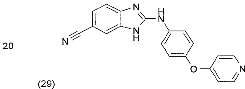
2-[4-(Pyridin-4-yloxy)-phenylamino]-3H-benzimidazol-5-carbonitril
